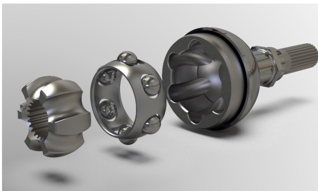
Typical Adlam Bell Joint exploded view
