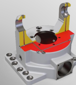
Wheel drive housing lubrication ports shown
